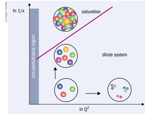
Fig. 3. The structure of the proton as a function of scale, Q^2 , and fractional momentum, x . The number of partons increases with Q^2 , but they have less momentum. The number of partons also increases as x decreases, to the point where the population is so dense that gluon recombination may lead to saturation. At low Q^2 the strong coupling \alpha_s is so large that reliable perturbative calculations are not possible.
