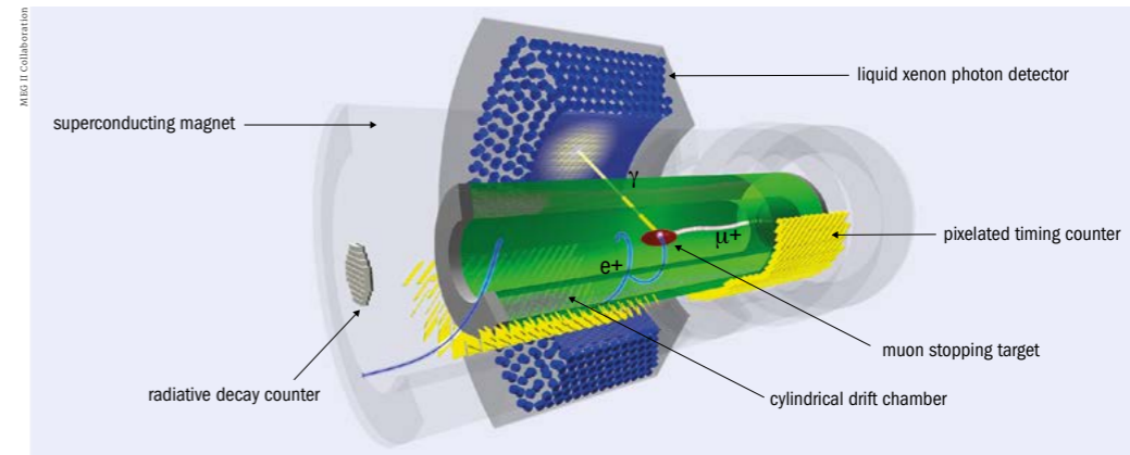
Fig. 2. Illustration of a \mu^+ \rightarrow e^+ \gamma event in MEG II.
