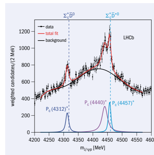
Fig. 1. The LHCb collaboration has discovered a new pentaquark, and resolved a previously discovered peak into two. The \Lambda_b^0 \rightarrow J/\psi p K^- data sample was fitted with three narrow resonances (blue, purple and cyan) plus a polynomial background.
