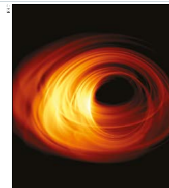
Black hole Matching the first image to a model. 10
