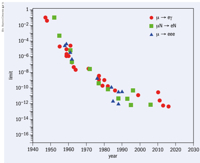
Fig. 1. Limits on the branching ratios of flavour-violating muon decays. In the mid 1950s, experiments using stopped pion beams improved on previous cosmic-ray limits, before experiments with stopped muons allowed further improvements in the mid 1970s. The current best limits in each channel were set by the MEG, SINDRUM-II and SINDRUM collaborations, respectively, each at PSI.
