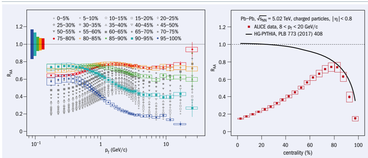
Fig. 1. Left: nuclear-modification factor versus p_T for 5% wide centrality classes, showing the suppression of high- p_T particle production in Pb–Pb collisions. The most peripheral 25% of ion collisions (coloured) exhibit completely different behaviour from the most central 75% (grey). Coloured bars show uncertainty on the normalisation. Right: mean R_{AA} (red) compared with a new model of suppression in peripheral collisions (black).
