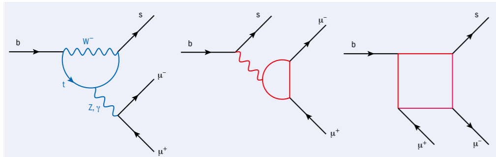
Fig. 4. Left: one of the Feynman diagrams giving the b \rightarrow s \mu^+ \mu^- transition in the SM. Middle and right: representative diagrams for models that generate b \rightarrow s \mu^+ \mu^- at one loop level, where the red lines correspond to particles beyond the SM.
