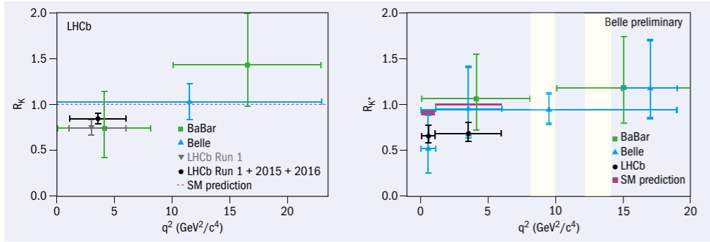
Fig. 3. The experimental results for R_{K^*} , measured in several bins of di-muon invariant mass squared, q^2 . The vertical faint yellow bands denote resonance regions that are cut out in the analyses.
