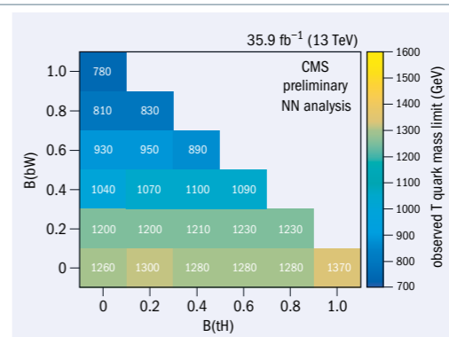
Fig. 1. Mass limits for T quarks in GeV. The limits are shown as a function of the probability to decay to a b quark and a W boson, versus the probability to decay to a top quark and a Higgs boson, assuming all other decays are to a top quark and a Z boson.
