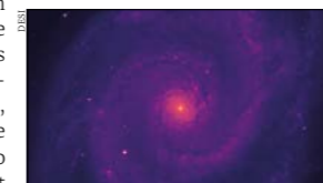
DESI captures the Whirlpool Galaxy.
