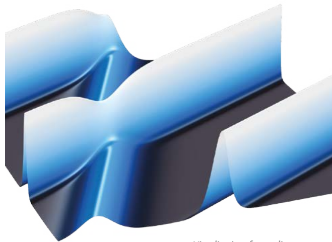
Visualization of two solitons colliding and reappearing in an optical fiber.
