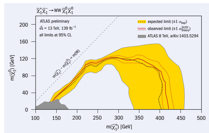
Fig. 1. New constraints (red) on a simplified SUSY model describing the production of a pair of charginos that both subsequently decay to a W boson and the lightest neutralino – a stable and invisible SUSY particle. The new sensitivity is significantly improved over that of the previous analysis (grey).
