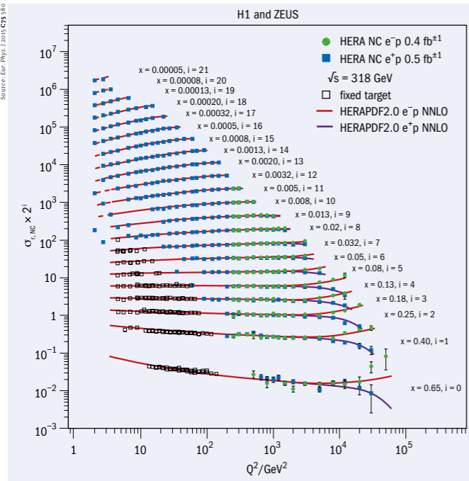
Fig. 1. HERA data on the e^+p scattering cross section is in close agreement with Standard Model predictions as a function of both scale, Q^2 , and the interacting parton's momentum fraction, x (the factor z^2 is artificially inserted to separate the curves vertically). At high x the cross section decreases with Q^2 because the parton distribution functions (PDFs) decrease as the partons give up their momentum by radiating gluons that split to quark-antiquark pairs, which radiate again. Correspondingly, the low- x PDFs increase.
