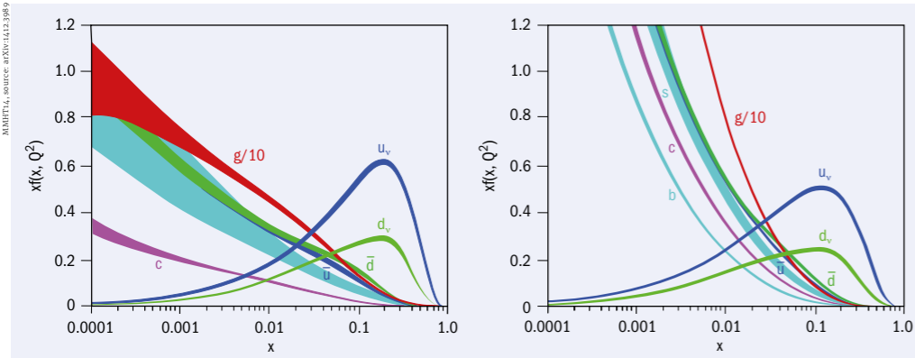
Fig. 2. The momentum distributions (PDFs) of all flavours of the partons at two scales ( Q^2 = 10 \text{ GeV}^2 , left, and 10^4 \text{ GeV}^2 , right). These curves are deduced from NNLO QCD fits to global hard-scattering data, with uncertainties arising from experimental errors and model assumptions.
