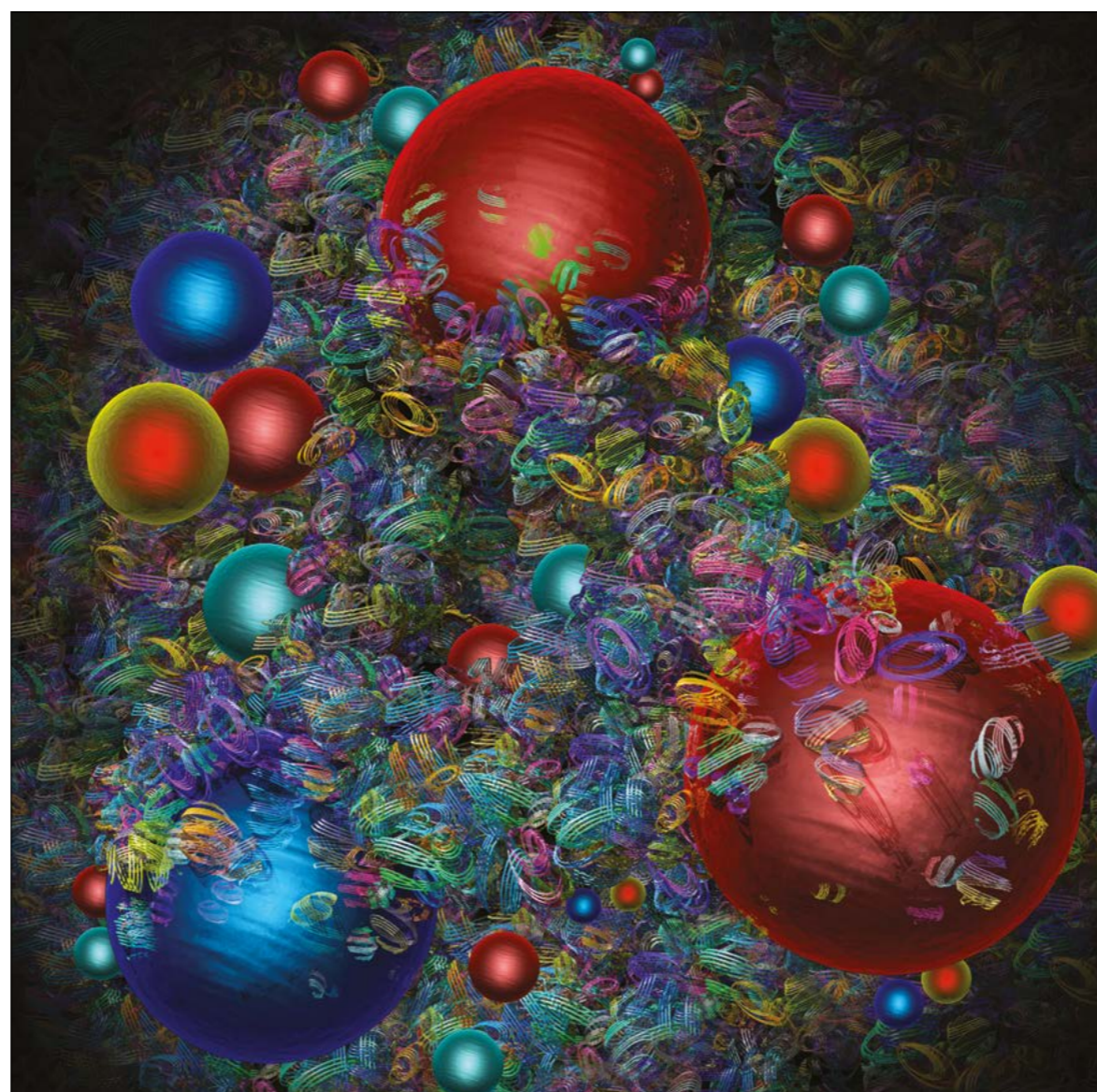
Glorious complexity An artist's impression of the mayhem of quarks and gluons inside the proton.
