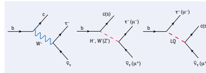
Fig. 1. The semileptonic decay of the b quark in the Standard Model (left). Possible new contributions to this process include exchanges of new colour-singlet states (middle), or new coloured states coupling simultaneously to quarks and leptons (right). The \bar{\nu}_\tau in b \rightarrow c\tau\bar{\nu}_\tau can also be replaced by a right-handed neutrino, which is not part of the Standard Model.
