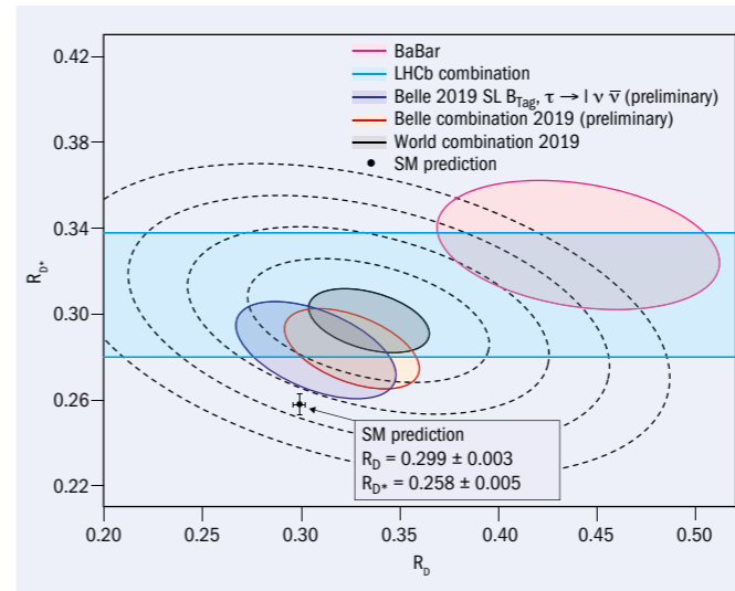
Fig. 2. Experimental results for the two observables probing lepton-flavour universality comparing b \rightarrow c\tau\bar{\nu}_\tau and b \rightarrow c\bar{l}\bar{\nu}_l decays, l=e, \mu . The point with error bars shows the SM prediction, while the shaded grey region shows the world experimental results average.
